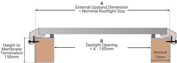
Figure 1: Fixed & Unventilated option directly fixed to builders upstand
