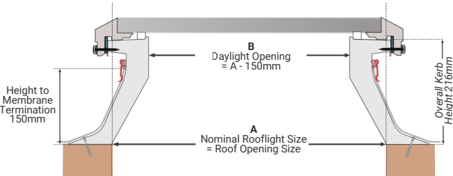
Figure 3: Rooflight with 150mm PVC kerb
